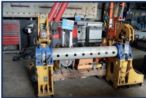
2000 Scorpion Break Out Make Up Tong, Model SSC 2000
