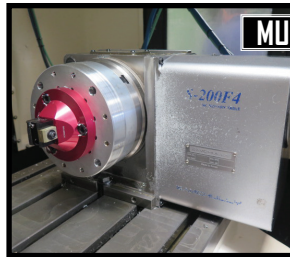
MUST SEE Samchully mdl. S-200F4 4 th Axis 8" Rotary Head
