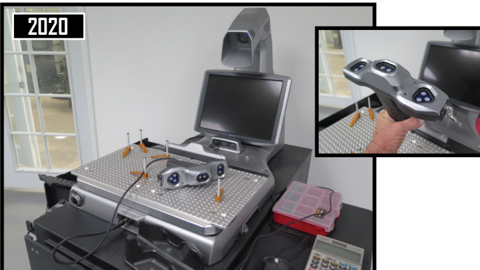
2020 Keyence XM-1200 Handheld Probe CMM Machine - Camera and Single Probe System w/Handheld Probe, M6 Fixture Plate
