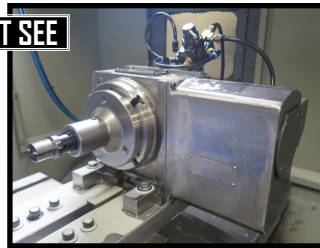
Samchully 4 th Axis 7" Rotary Head w/ 5C Pneumatic Closer
