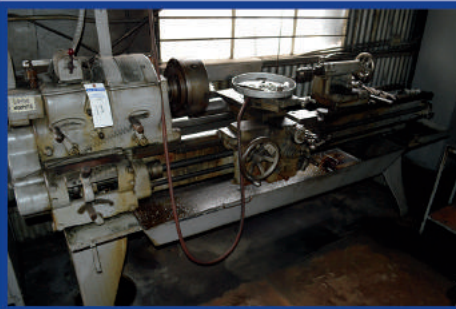
Leblond Regal Lathe 16", 10" Chuck, Tailstock, 64" Centers, Assorted Boring bars and Accessories, Small Grey Cabinet with Contents Included
