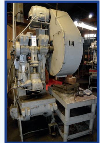
Niagara A3 Punch Press, 45 Ton, 4" Stroke, 12.25" Shut Height, 2.25" Adjustment, With Steel Table and All Included Contents
