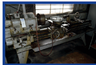
Leblond Regal Lathe 16", 10" Chuck, Tailstock, 64" Centers
